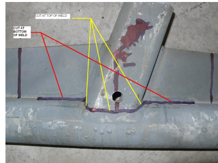
Stem/Bail connection before mod
