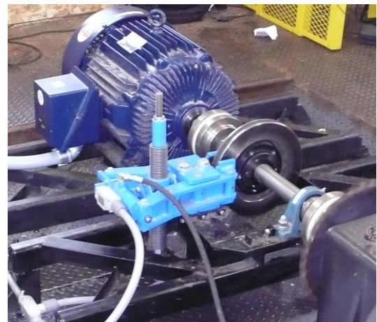
Installed Caliper Brake
