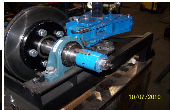
Caliper Brake During Testing
