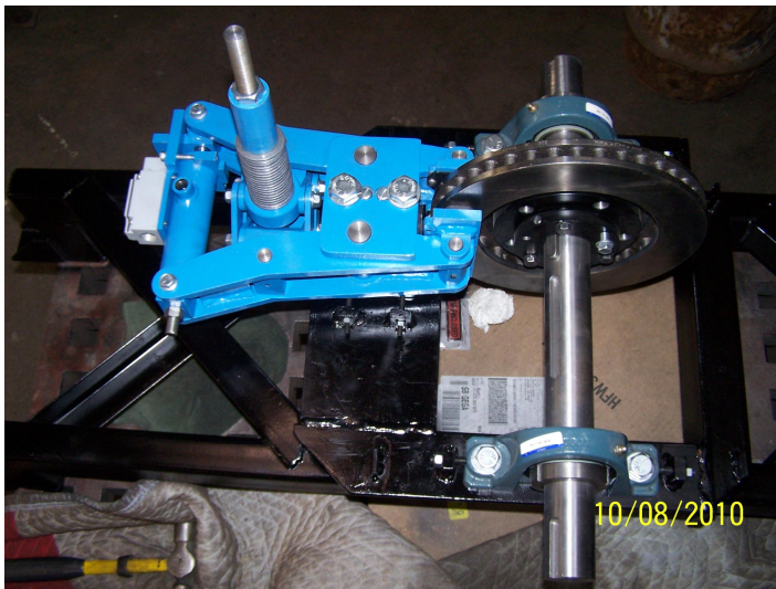
Caliber Brake Fully Assembled W/ Brake Disc
