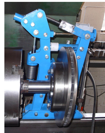
Service Brake in Testing
