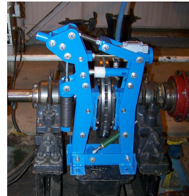
Installed Service Brake
