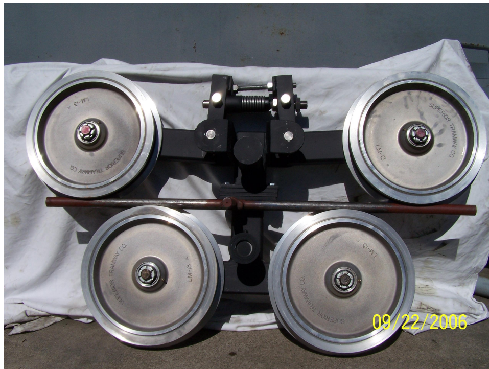
LM-67 Assembly with LM-01 Sheave Frame
